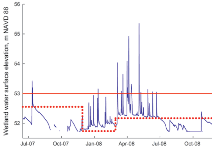
Figure 3. Stage hydrograph for wetland during period of interest. Crest of weir at downstream (river) end of wetland is shown as solid red line, and the elevation of adjustable stoplog crest is shown as the red dotted line.
