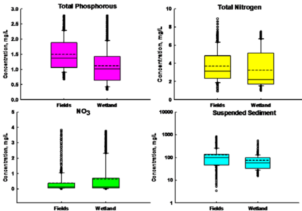
Figure 4. Box and whisker plots for selected water quality constituent concentrations of samples collected from the primary inflow to the managed wetland, a slough that conveyed runoff from about 100 ha of cultivated fields (labeled “Fields”), and for samples collected from the downstream end of the wetland (labeled “Wetland”). Medians of all constituents except for NO 3 -N were significantly different ( P < 0.013 )
